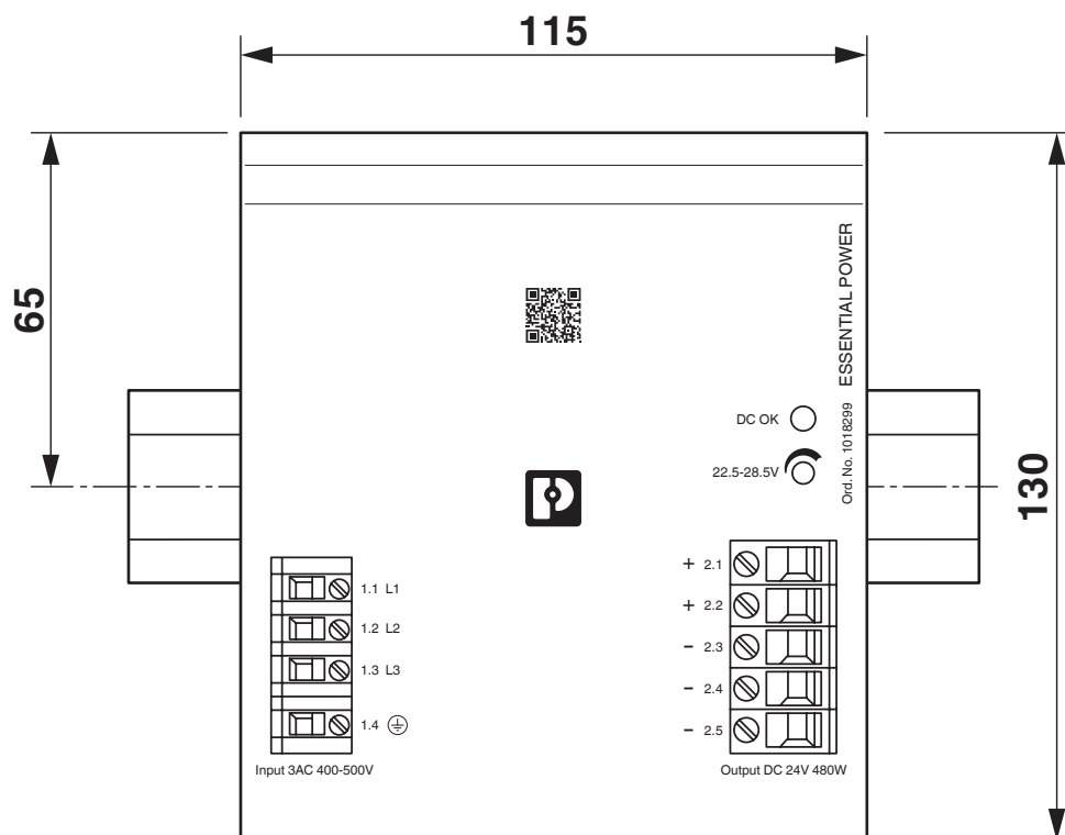
Dimensional drawing
