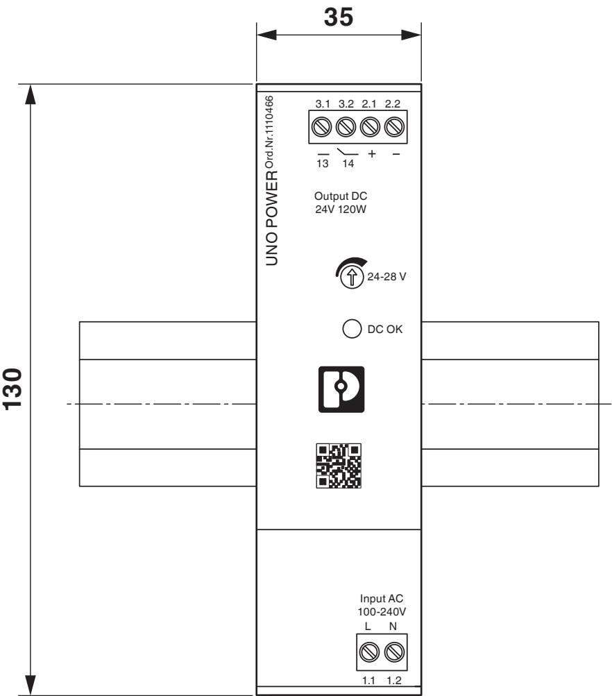
Dimensional drawing
