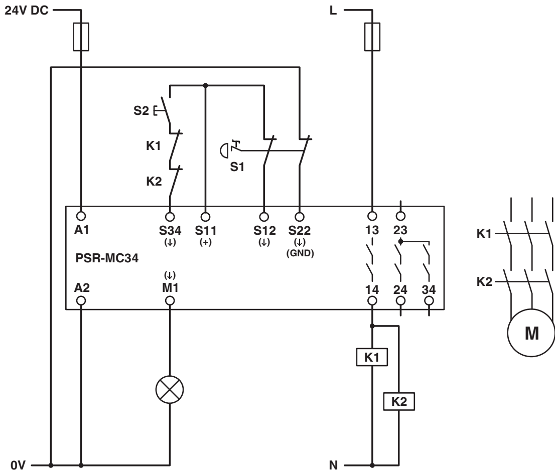
Circuit diagram
