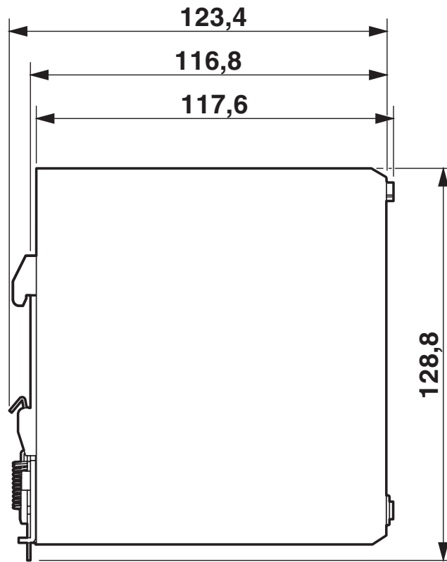
Dimensional drawing
