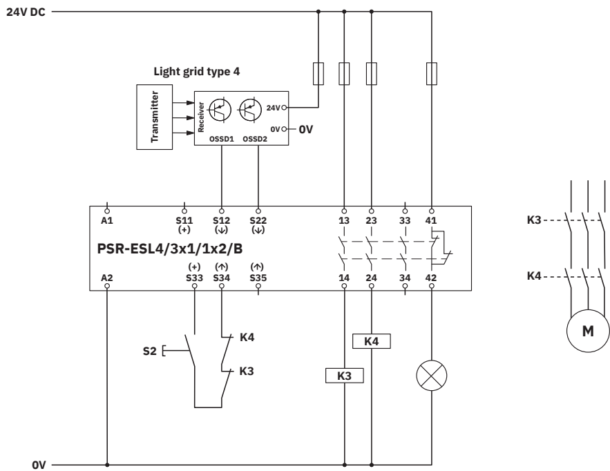
Circuit diagram
